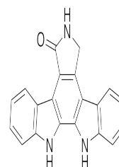
Chemical structure of K252c
