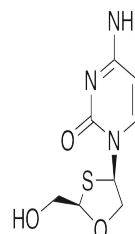
Chemical structure of Lamivudine
