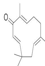
Chemical structure of Zerumbone
