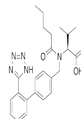
Chemical structure of Valsartan
