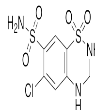
Chemical structure of Hydrochlorothiazid...
