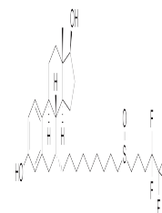
Chemical structure of Fulvestrant
