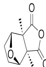
Chemical structure of Cantharidin
