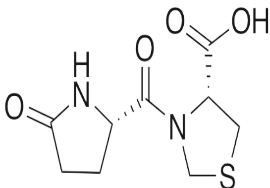
Chemical structure of Pidotimod
