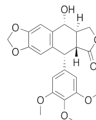
Chemical structure of Podophyllotoxin
