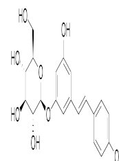
Chemical structure of Polydatin
