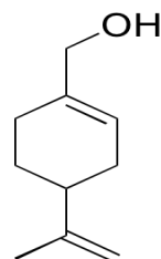
Chemical structure of Perillyl Alcohol
