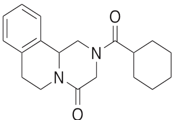
Chemical structure of Praziquantel
