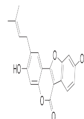
Chemical structure of Psoralidin
