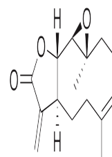
Chemical structure of Parthenolide
