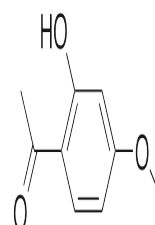
Chemical structure of Paeonol
