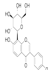
Chemical structure of Puerarin
