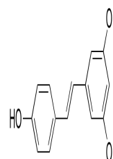
Chemical structure of Resveratrol
