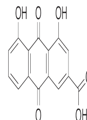
Chemical structure of Rhein
