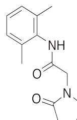
Chemical structure of Nefiracetam
