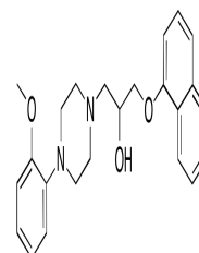
Chemical structure of Naftopidil
