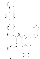
Chemical structure of Naringin
