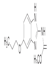
Chemical structure of Oxibendazole
