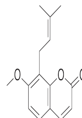
Chemical structure of Osthole
