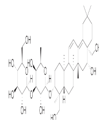
Chemical structure of Saikosaponin B2
