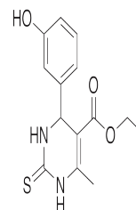
Chemical structure of Monastrol
