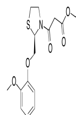
Chemical structure of Moguisteine
