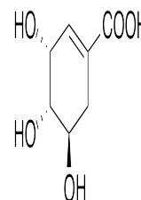
Chemical structure of Shikimic Acid
