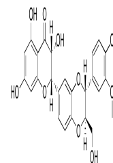
Chemical structure of Silymarin
