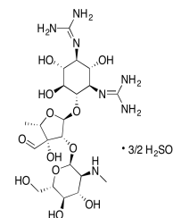
Chemical structure of Streptomycin Sulfate...
