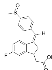
Chemical structure of Sulindac
