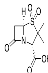
Chemical structure of Sulbactam
