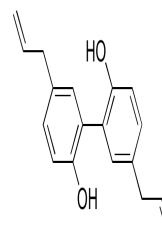
Chemical structure of Magnolol
