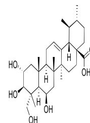
Chemical structure of Madecassic Acid
