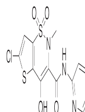
Chemical structure of Lornoxicam
