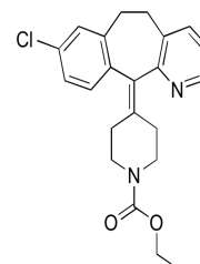
Chemical structure of Loratadine
