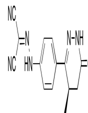
Chemical structure of Levosimendan
