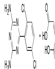
Chemical structure of Irsogladine Maleat...
