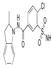
Chemical structure of Indapamide
