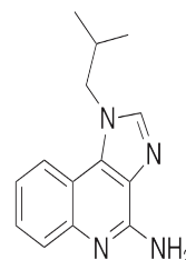
Chemical structure of Imiquimod
