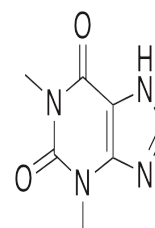
Chemical structure of Theophylline
