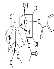
Chemical structure of Hypaconitine
