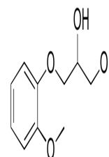
Chemical structure of Guaifenesin
