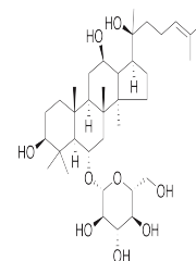
Chemical structure of Ginsenoside Rh1
