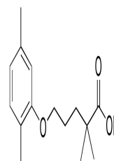
Chemical structure of Gemfibrozil
