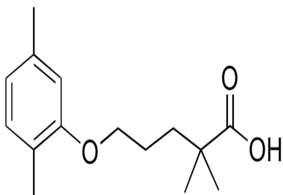
Chemical structure of Gemfibrozil
