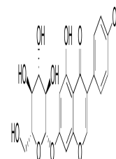
Chemical structure of Genistin
