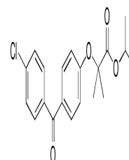
Chemical structure of Fenofibrate
