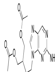
Chemical structure of Famciclovir
