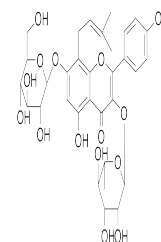
Chemical structure of Icariin
