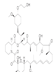
Chemical structure of Everolimus
