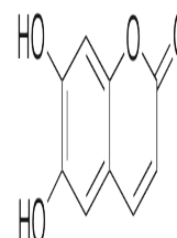
Chemical structure of Esculetin
